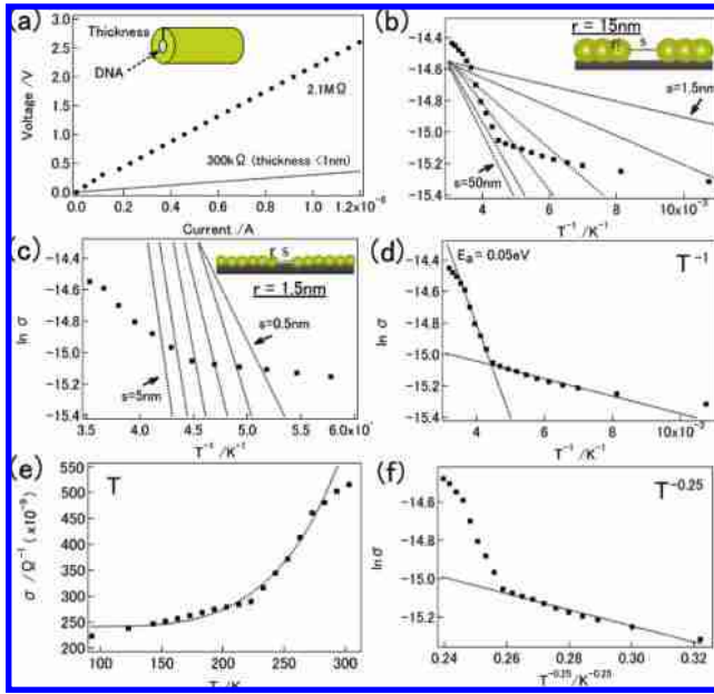
Figure 2. Electrical conduction measurement results of the metallized DNA. (a) The I – V curve of the single metallized DNA measured at T = 293 K. The lower dotted line corresponds to the theoretical resistance of a single cylindrical gold nanowire (see Supporting Information). Panels b–f are the temperature dependence of the electrical conductance. The dotted lines in (b) and (c) are temperature dependence of the theoretical electrical conductivity of the discontinuous gold films whose radius of the metal is 15 and 1.5 nm, respectively. The theoretical curves in (b) are generated when the gap size is 1.5, 3, 7.5, 15, 30, and 50 nm (the electrical conductivity decreases as the gap size increases). Further, the curves in (c) are obtained when the gap size is 0.5, 1, 1.5, 3, 5, and 10 nm. On the other hand, the dotted lines in panels d, e, and f are the theoretical curve obtained by the Arrhenius equation, small polaron hopping theory, and Mott variable range hopping theory, respectively.
