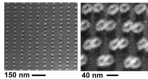
FIG. 10. Images of divots written in a polymer film using heat and force applied by a silicon atomic-force-microscope (AFM) cantilever. The images are recorded using the same cantilever used during the writing process and a thermal reading technique involving heat conduction from the cantilever into the substrate (Ref. 53).
